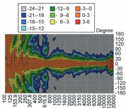
Directivity vertical 2D 1
