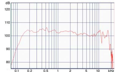
Frequency Response
