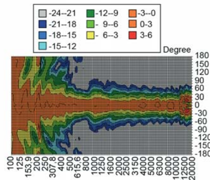
Directivity horizontal 2D 1
