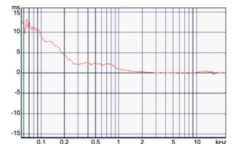
Group Delay
