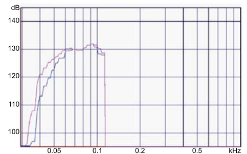
Max SPL (blue = 3% purple = 10%)
